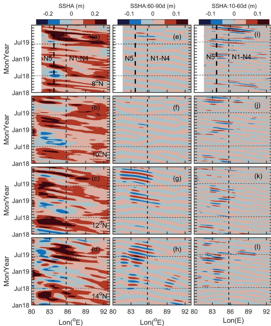
Figure 9. Time -longitude plots (Hovmöller diagrams) of AVISO SSHA at mooring locations, where rows from top to bottom represent 8^{\circ}\text{N} , 10^{\circ}\text{N} , 12^{\circ}\text{N} , and 14^{\circ}\text{N} . Left (a, b, c, d), middle (e, f, g, h), and right (i, j, k, l) columns display unfiltered SSHA, 60-90-day band-passed filtered SSHA, and 10-60-day band-passed filtered SSHA, respectively. The thin dashed and thick dashed vertical lines represent longitudinal position of N1-N4 and N5, respectively. Thin dashed horizontal lines are the start and end of mooring observations
