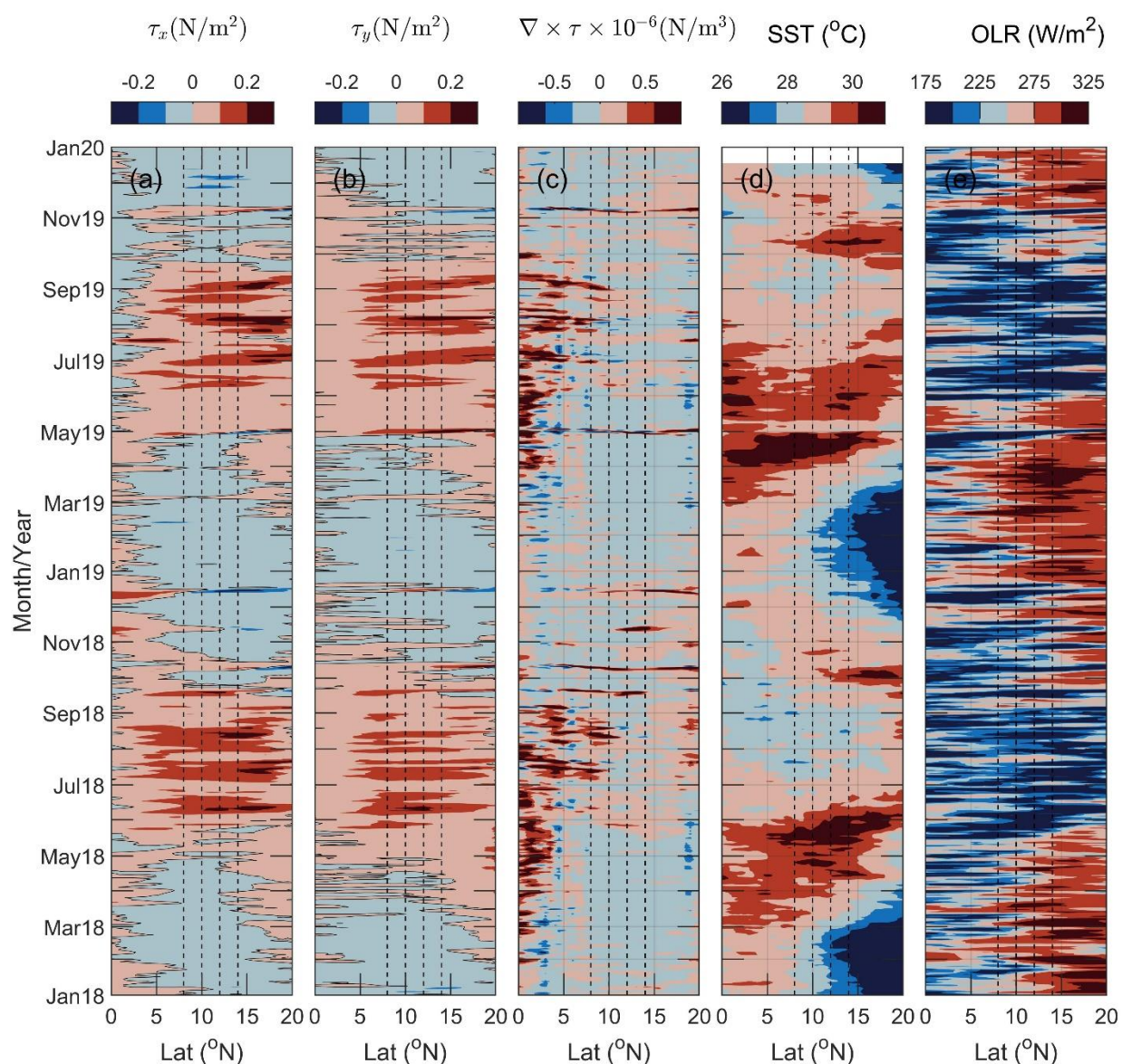
Figure 4. Latitude-time plot of longitudinally-averaged (between 84° E and 90° E) surface zonal stress ( \tau_x ) (a), meridional stress ( \tau_y ) (b), wind-stress curl ( \nabla \times \tau ) (c) from ERA5 reanalysis products from https://www.ecmwf.int/en/forecasts/datasets/reanalysis-datasets/era5 , and sea surface temperature (SST) (d) from https://psl.noaa.gov/ , and outgoing longwave radiation (OLR) (e) from the Climate data Record (CDR), https://climatedataguide.ucar.edu/climate-data/outgoing-longwave-radiation-olr-hirs . Plots were constructed from daily averaged wind stress, SST, and OLR. Thin black lines in (a) and (b) represent zero stress contours. Vertical dashed lines are the meridional positions of NRL moorings.
