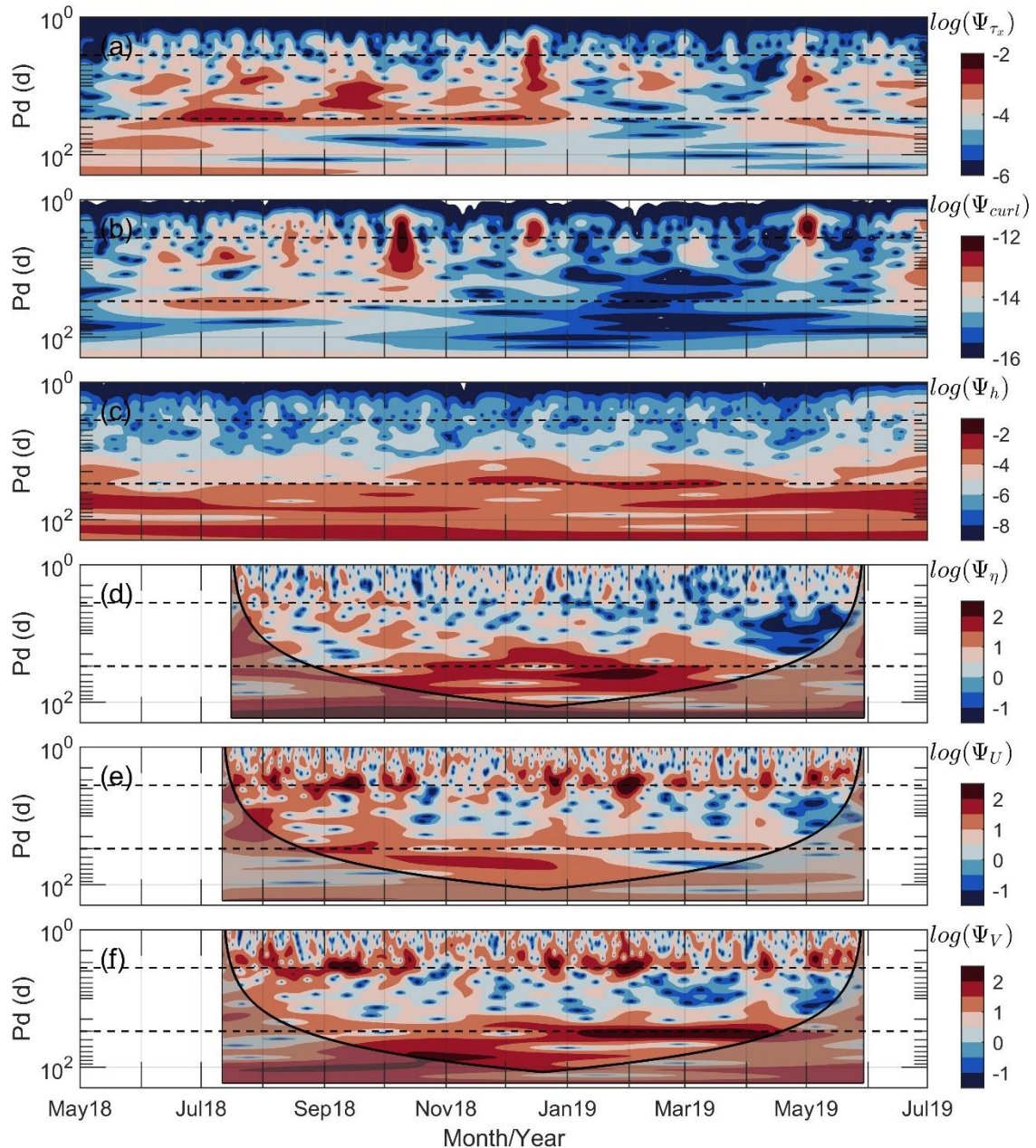
Figure 10. Wavelet spectra at N1 plotted as a function of period ( p_d ) and time ( t ): (a) zonal wind stress, \Psi_{\tau_x}(t, p_d) ( \text{Nm}^{-2} ) 2 and (b) wind-stress curl, \Psi_{curl}(t, p_d) ( \text{Nm}^{-3} ) 2 from hourly ERA5, (c) SSH anomaly, \Psi_h(t, p_d) ( \text{m}^2 ) from daily AVISO, (d) 26^\circ\text{C} isotherm displacement, \Psi_\eta(t, p_d) ( \text{m}^2 ) from hourly-averaged moored thermistor measurements, (e) zonal velocity, \Psi_U(t, p_d) and (f) meridional velocity, \Psi_V(t, p_d) ( \text{m s}^{-1} ) 2 at 120 m from hourly-averaged ADCP currents. Thin dashed lines are inertial frequencies (top line) and 30-day periods (bottom line).
