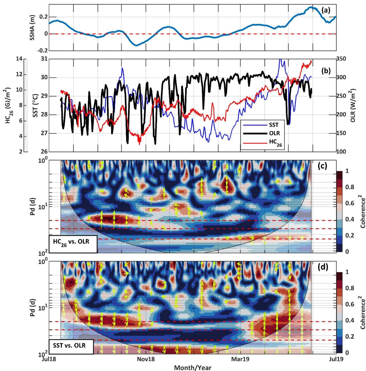
Figure 18. Time series of SSHA (thick blue line) at N4 (a), heat content above the 26°C isotherm ( HC_{26} ) (red line), SST (blue line), and OLR (thick black line) (b). The squared wavelet coherence between heat content and OLR (c) and SST and OLR (d) are plotted as a function of time and period. Arrows indicate the relative phase between HC_{26} and OLR and between SST and OLR with in-phase pointing right, anti-phase pointing left, HC_{26} or SST leading OLR by 90 degrees pointing straight down, and HC_{26} or SST lagging OLR by 90 degrees pointing straight up. The red dashed lines are at 20-d, 30-d, and 50-d periods.
