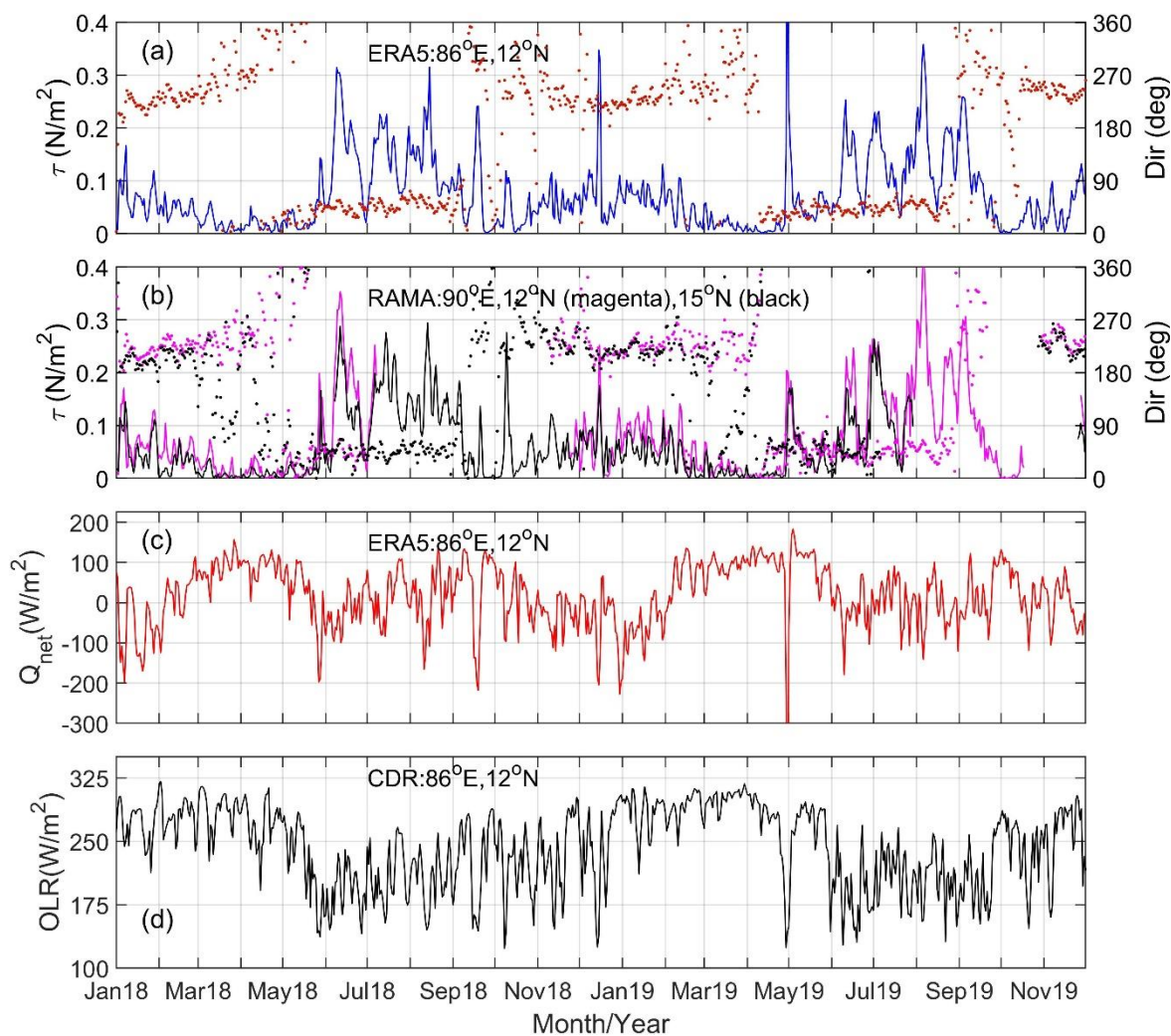
Figure 5. (a): Time series of daily-averaged surface wind-stress magnitude ( \tau ) (blue line) and direction (Dir) (red dots) at 85.75° E, 12° N (N3 site) from ERA5 model output. (b): Daily-averaged wind stress (solid lines) and direction (dots) at 90° E, 12° N and 15° N from RAMA buoy measurements, where magenta and black colors represent 12° N and 15° N, respectively. Buoy measurements at 12° N and 15° N were combined to construct a two-year time series. (c): Daily-averaged net surface-heat flux ( Q_{net} ) at 12° N, 86° E from ERA5 model output. (d): Daily-averaged outgoing longwave radiation (OLR) at 12° N, 86° E from CDR developed by NOAA and University of Maryland. Here the direction of the wind is where the wind is originating, and downward net-heat flux is positive, and the OLR (upward flux) is positive.
