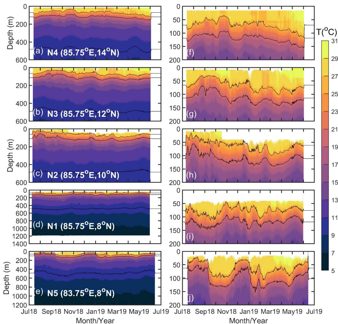
Figure 3. Time-depth sections of hourly-averaged temperature at N1-N5. The right panel displays an enlarged view of temperature variability in the thermocline. The black lines are two-day low-passed (de-tided) isotherms of 10° C, 20° C, and 26° C. Only 20° C and 26° C isotherms are marked in the right panels. Approximate locations of moorings are given in parenthesis.
