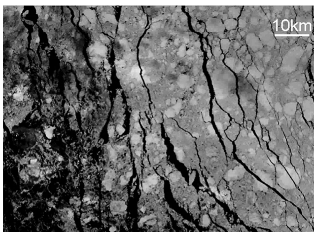
Figure 19. A subsene of Landsat8 image L7 (L780920) showing refrozen floes and leads.
