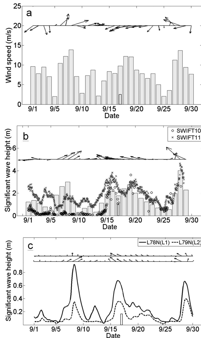
Figure 7. Same as in Figure 6 except near the Landsat8 images L1 and L2 at (165°W, 76°N). The vector plots are arranged from bottom to top to correspond to L1 and L2, respectively. The hollow vertical bar in each figure marks the date of both images (17 September).
