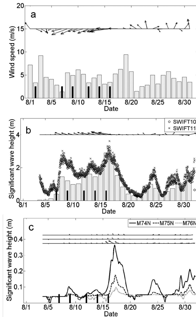
Figure 6. (a) Surface wind speed and direction from NCEP at the ice edge (150°W, 72°N) near the MEDEA and the RADARSAT-2 images. (b) Significant wave height and direction from WW3 at the same ice edge location superimposed with SWIFT wave height. (c) Significant wave height and direction from WW3 at the three MEDEA image locations. The vector plots are arranged from bottom to top to correspond to 74°N, 75°N, and 76°N, respectively. The vertical dark bars in each figure mark the dates of MEDEA images.
