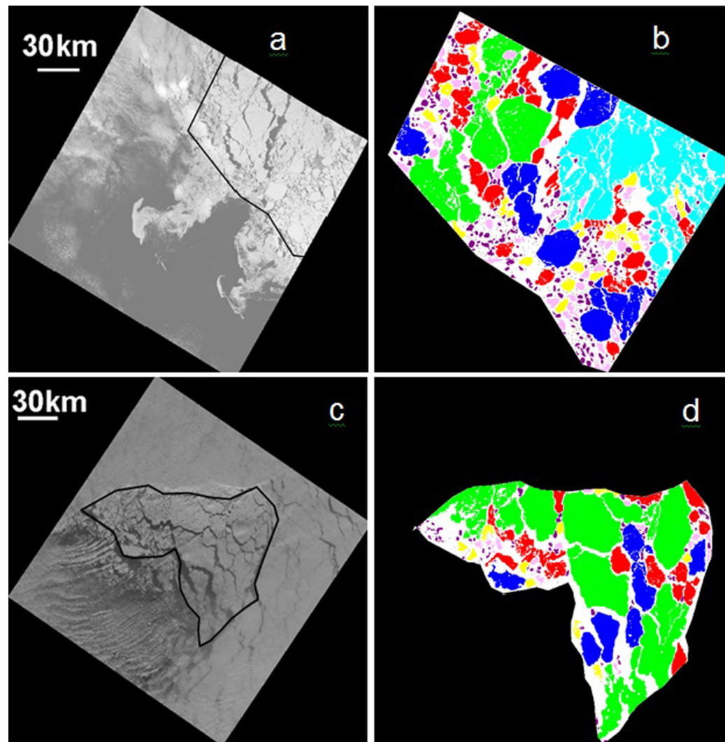
Figure 14. Input and output images of Landsat8 showing transitional development between floes and leads. (a, b) L73N0926 (L5); (c, d) L76N0919 (L3). The analyzed regions are marked in each image.
