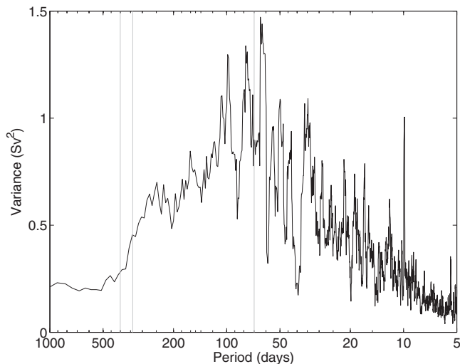
Fig. 5. Variance preserving power spectra ( Sv^2 ) of the 20-year global HYCOM reanalysis transport time series through Kerama Gap. Vertical lines show the boundaries of the temporal bands investigated, i.e. 70, 345, and 400 days.
