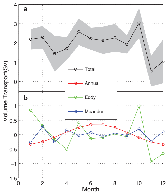
Fig. 6. (a) Seasonal cycle of transport through Kerama Gap and (b) the contribution of different signals to the transport seasonal cycle from the 1/12.5^\circ global HYCOM reanalysis. The shaded area in (a) represents the seasonal cycle uncertainty and the dashed line shows the 20-year mean transport. (For interpretation of the references to color in this figure, the reader is referred to the web version of this article).
