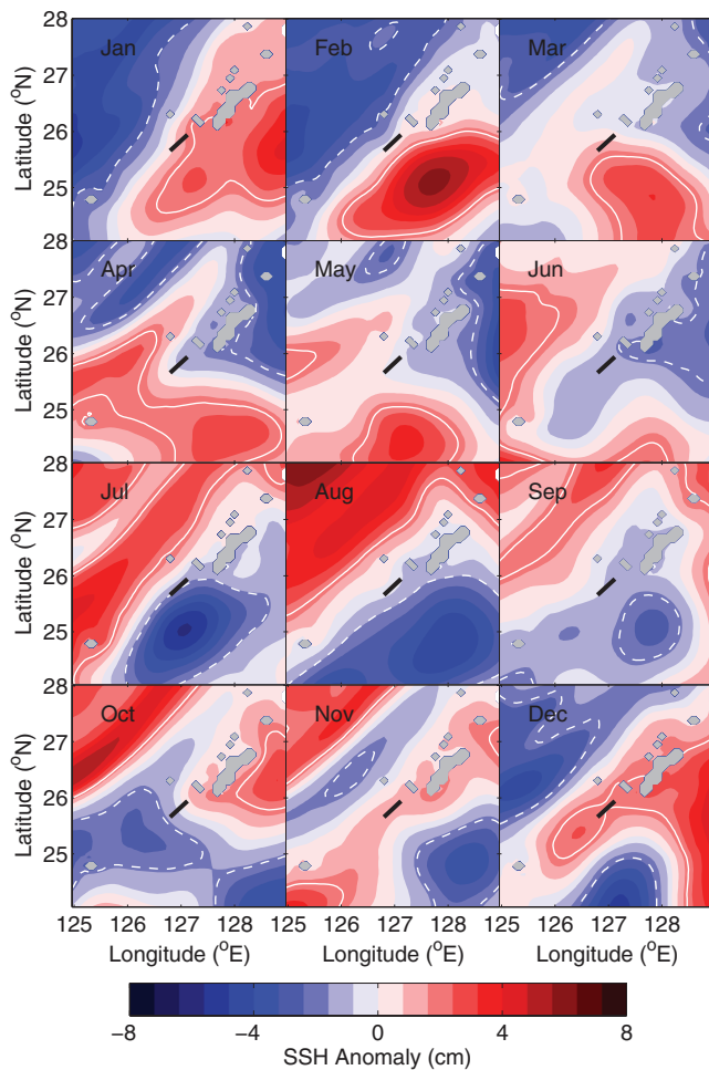
Fig. 11. Monthly mean (1993–2012) SSHA (cm, relative to annual mean SSH with annual steric effect removed) pattern from January to December. Contours with SSHA = 2 cm (solid white line) are used to identify the anomalous anticyclones and contours with SSHA = -2 cm (dashed white lines) are used to identify the anomalous cyclones.
