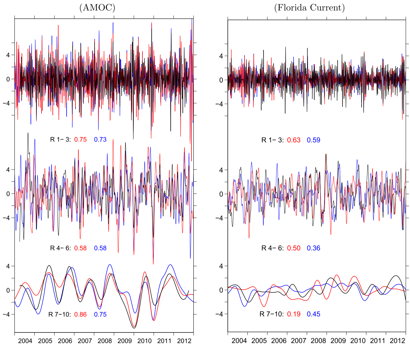
Figure 6. Similar to the Figure 5 but the intrinsic mode functions (IMFs) are summed to illustrate the variability on three general time scales: a) high frequency (IMFs 1–3, period of 3 weeks or shorter); (b) intraseasonal (IMFs 4–6, period of 1–6 months); and (c) seasonal and interannual (IMFs 7–10).
