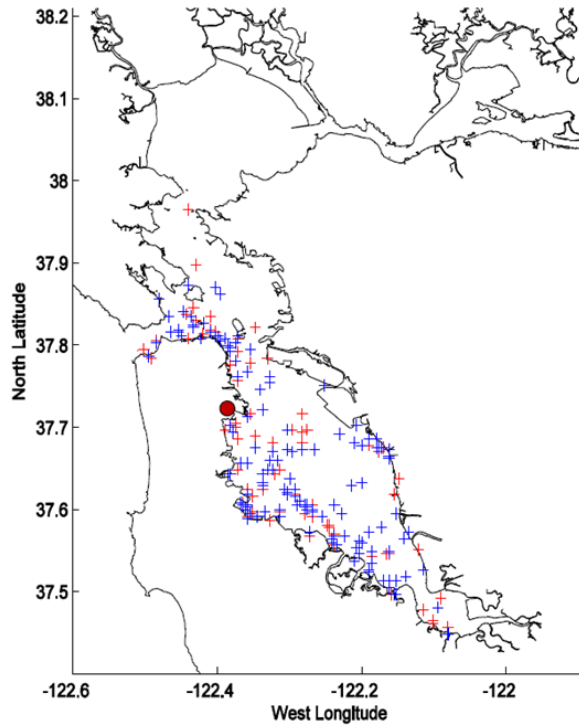
Figure 5.2. Particle tracking results for San Francisco Bay. A. Particle distributions near Hunters Point computed by a particle tracking algorithm for Jan. 2004. Particles were released at the locations indicated by the circles. B. Particle distribution in San Francisco Bay after 15 days (red pluses) and 28 days (blue pluses) for Feb. 2004. The hydrodynamic forcing is from the NCOM SFB grid (300 m). One particle was released every 24 hr just south of HPS (red circle).
