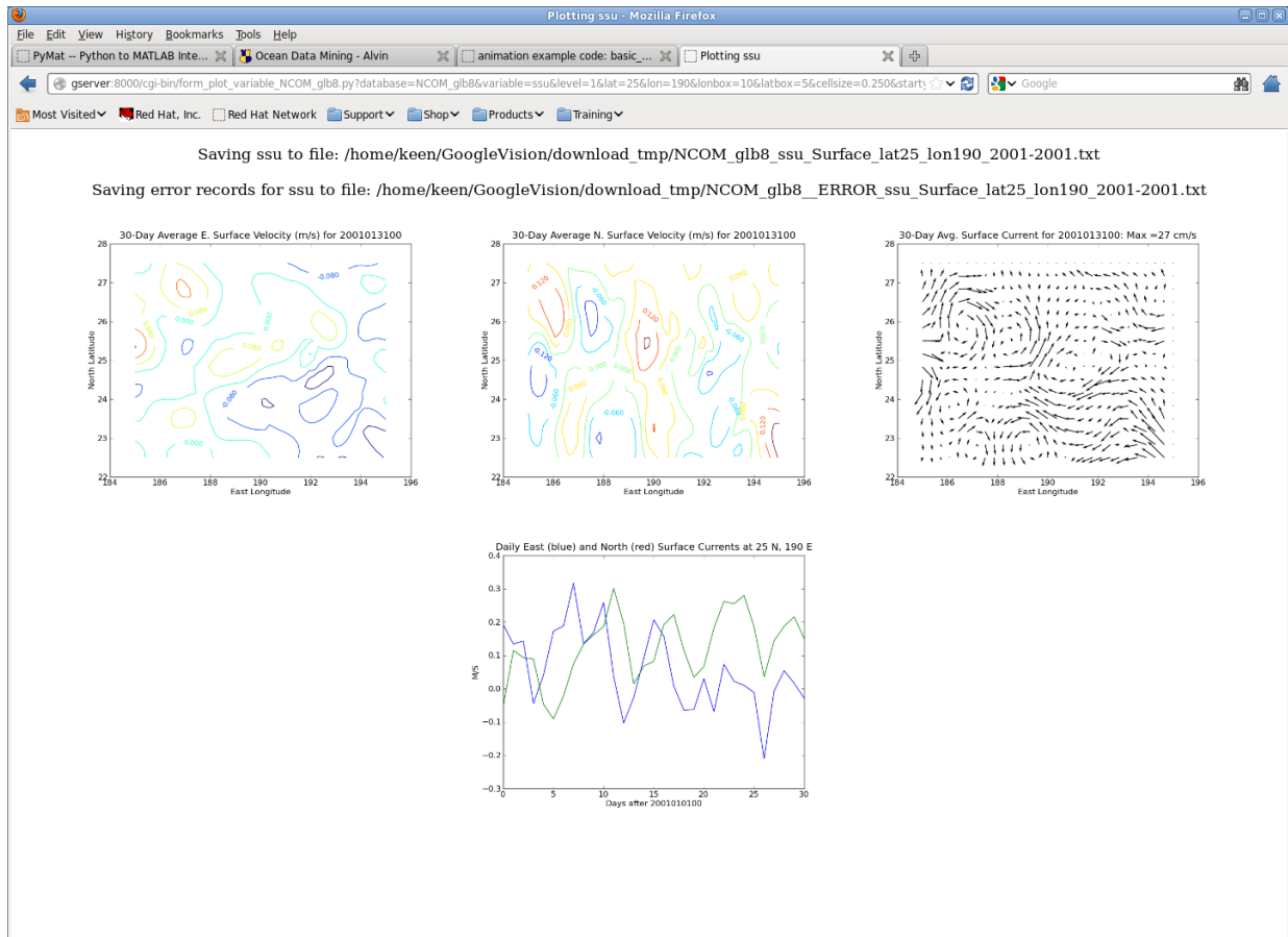
Figure 4.16. Example of output from the NCOM global 1/8^\circ database.
