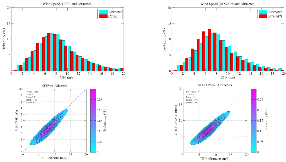
Figure 4-1: WW3 U 10 wind speed probability: CFRS (left) and NOGAPS (right) compared to altimeter winds.
