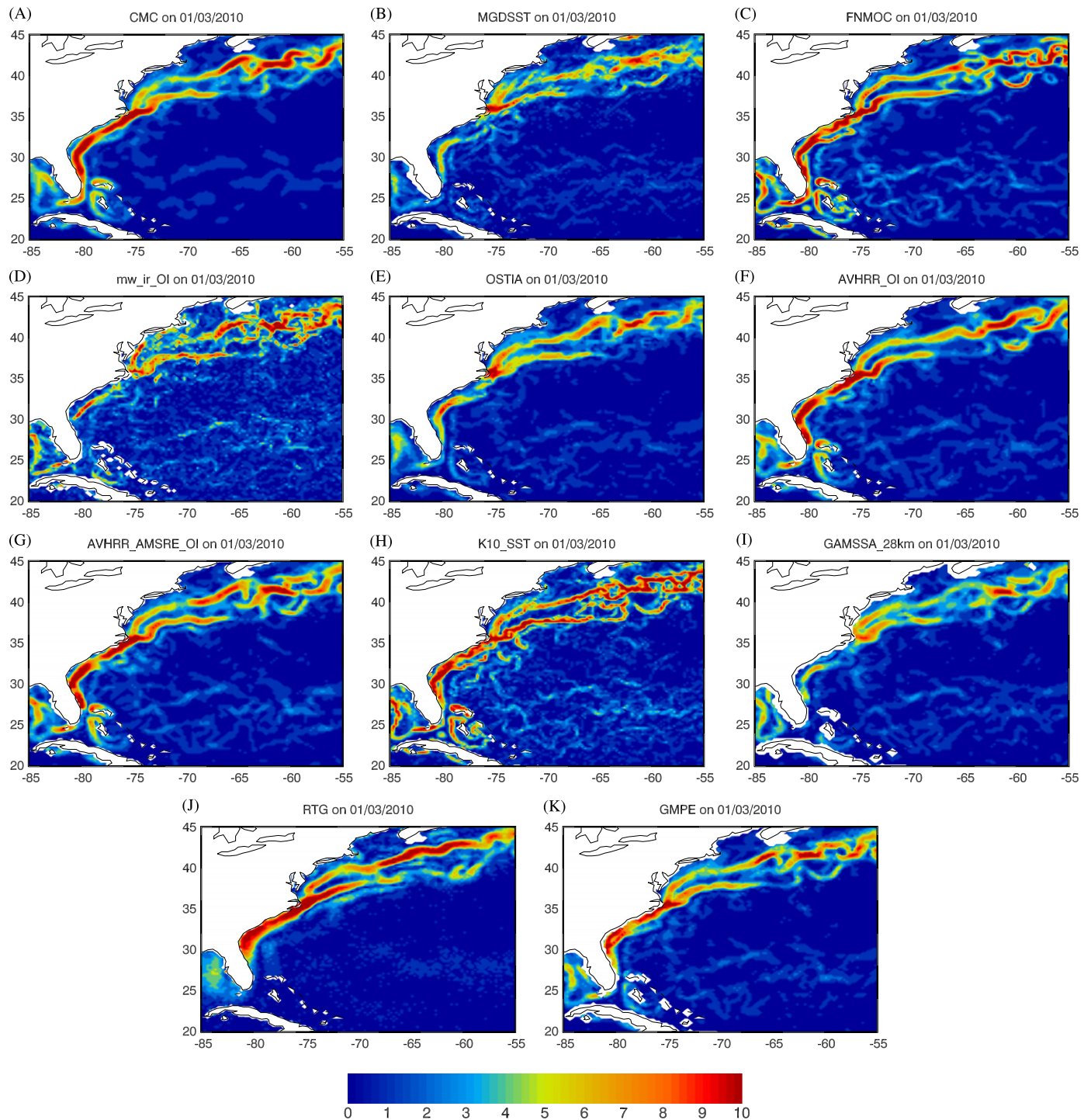
Fig. 3. Averaged east–west, north–south gradients of SST ( \text{K } 100 \text{ km}^{-1} ) in the Gulf Stream region on 1st March 2010 for (A) CMC, (B) MGDSST, (C) FNMOC, (D) RSS MW/IR, (E) OSTIA, (F) OISST.v2 AVHRR, (G) OISST.V2 AMSR/AVHRR, (H) NAVO K10, (I) GAMSSA, (J) RTG, and (K) GMPE median.
