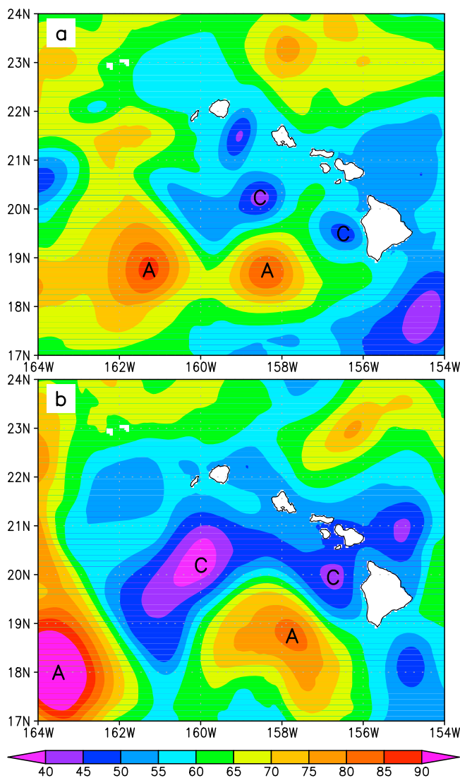
Figure 8. SSH (cm) on 10 September 2009 from (a) the QSCAT experiment and (b) the NOGAPS experiment.
