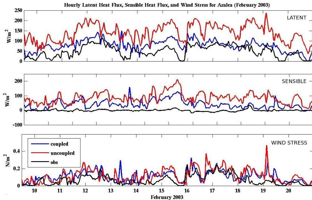
Figure 1-10: Hourly latent and sensible heat fluxes ( W/m^2 ) and wind stress ( N/m^2 ) for the fully-coupled COAMPS run and observations at Azalea.
