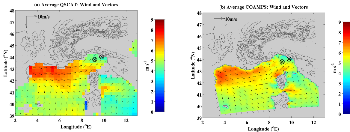
Figure 2-2: Near-surface winds over the Ligurian Sea. (a): Monthly average of neutral
