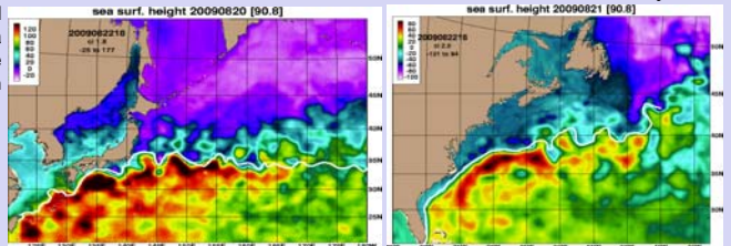
Frontal analysis < 4 days old = white, analysis ≥ 4 days old = black The frontal analysis is performed at the Naval Oceanographic Office
