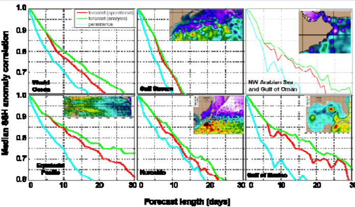
Green line: Analysis quality atmospheric forcing throughout the forecast period Red line: Atmospheric forecast for first 5 days, then gradually reverting toward climatology
