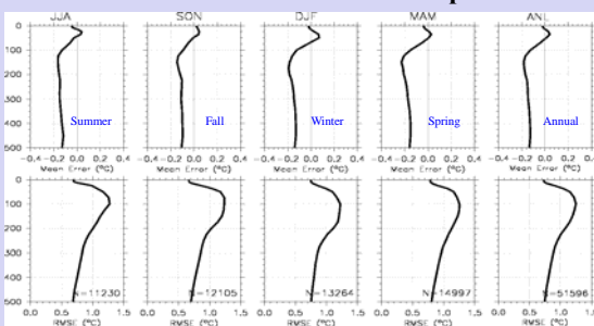
Temperature (°C) vs. depth error analysis in the upper 500 m against unassimilated profiles for the region 70°S to 50°N. The top and bottom rows are mean error and RMSE, respectively. The number of unassimilated profiles used in each season is indicated in the bottom row. This is the number of near-surface observations used and this value decreases with depth since not all profiles exist down to 500 m depth.
