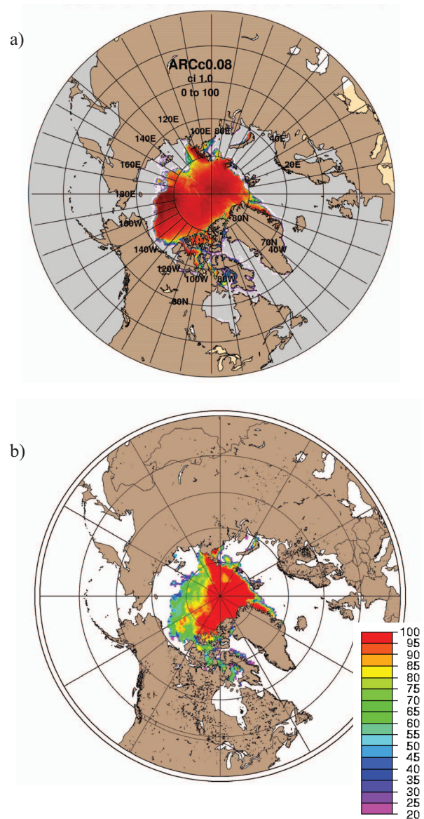
Figure 3. Ice Concentration (in percent) from a) HYCOM/NCODA/CICE data assimilation and b) SSM/I. Images valid for 03 August 2007.
