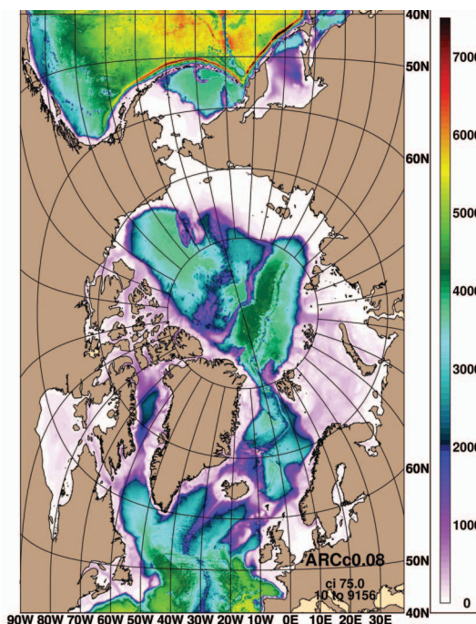
Figure 1. 1/12°HYCOM/CICE Arctic Ocean bathymetry (m).
