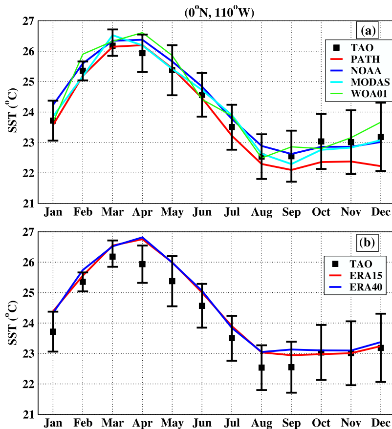
Figure 12. Climatological mean of SST time series at (0°N, 110°W) located in the eastern equatorial Pacific. Monthly SST climatology from the TAO buoy is also shown for comparison purposes. Also shown are the confidence limits at 95% based on the standard error of the SSTs from the TAO buoy.
