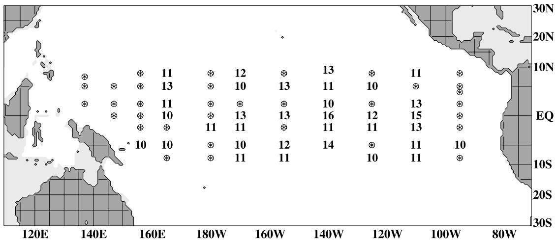
Figure 10. Locations of the moored buoys from the TAO array where monthly mean SST climatologies were constructed to compare with climatological SSTs from the six products described in section 2. The number of years which are used for forming monthly climatologies is indicated by a two-digit number.
