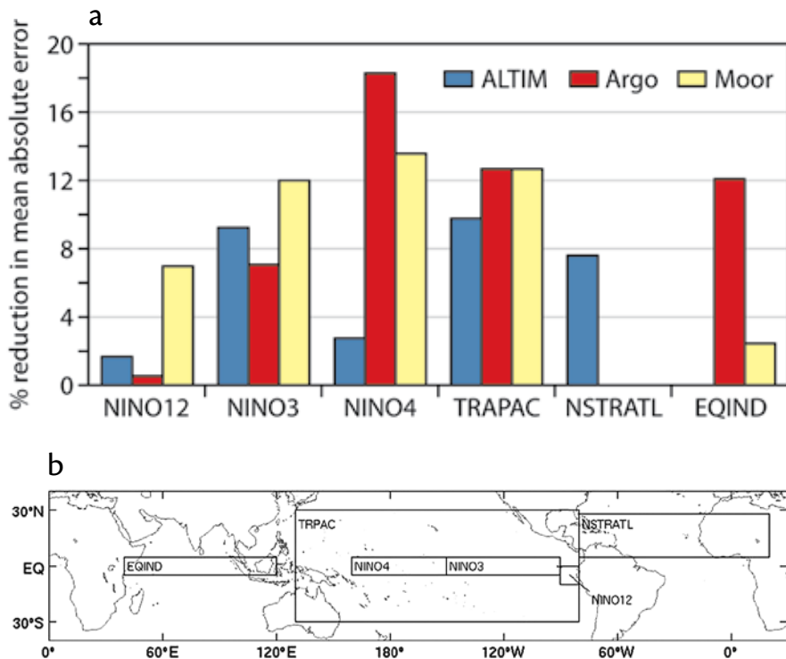
Figure 3. (a) Percentage reduction in the mean absolute error of one- to seven-month SST forecasts for the period 2001–2006. ALTIM, Argo, and Moor refer to the difference between the mean absolute error when altimeter, Argo, and mooring data are withheld, respectively. Results are presented for the regions denoted in (b).
