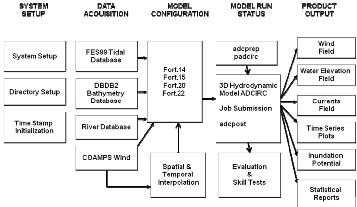
Figure 1. Schematic diagram of RELO-ADCIRC system
