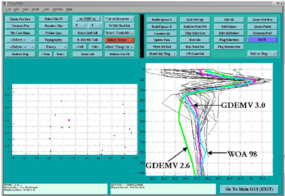
Figure 5. Screen shot from the ODDESA profile editor showing observed (black dots and black lines) and climatological (thick colored lines) salinity in the tropical north central Pacific Ocean. The GDEMV-2.6 profile overshoots the minimum due to the method for splicing upper (0 to 400 m) and mid-depth profiles together.
