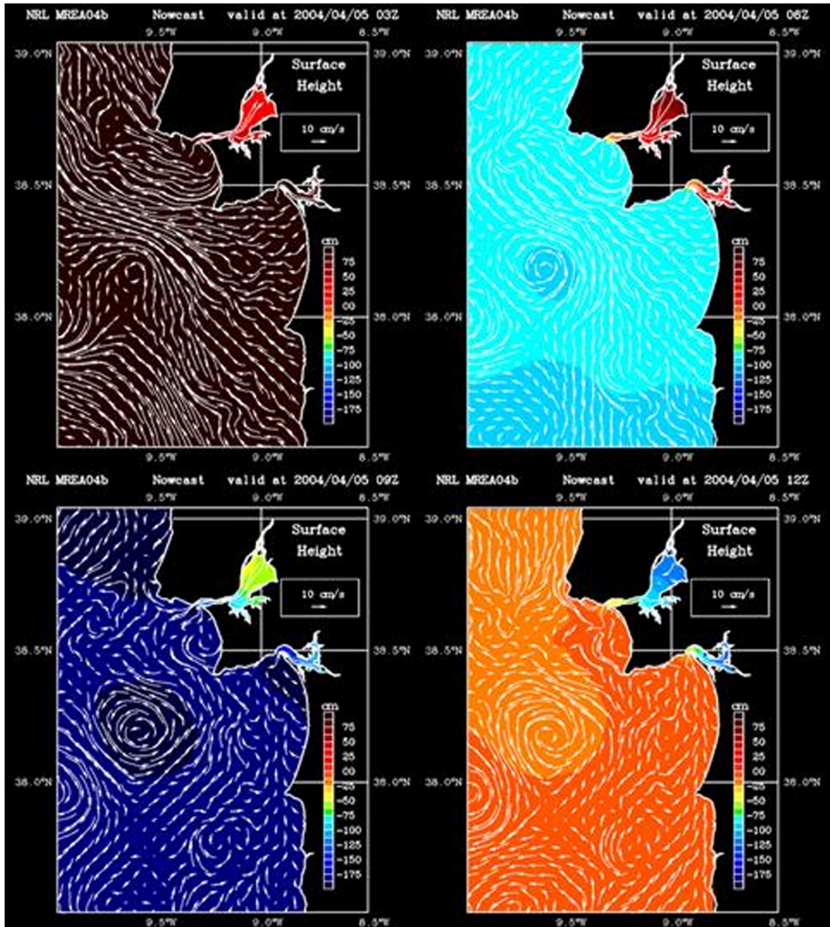
Fig. 6. The model sea level predictions at 3-h intervals (in color) show the tidal phase to be quite uniform for the region except in the bay areas. The model surface current vectors are overlaid. (For interpretation of the references to color in this figure legend, the reader is referred to the web version of this article.)
