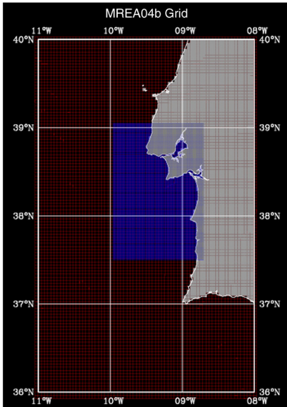
Fig. 1. A nested grid system was applied to the MREA04 sea trial region off Portuguese coast. The host grid (in red) has a 4-km resolution and the nested grid (in blue) a 1-km resolution. (For interpretation of the references to color in this figure legend, the reader is referred to the web version of this article.)
