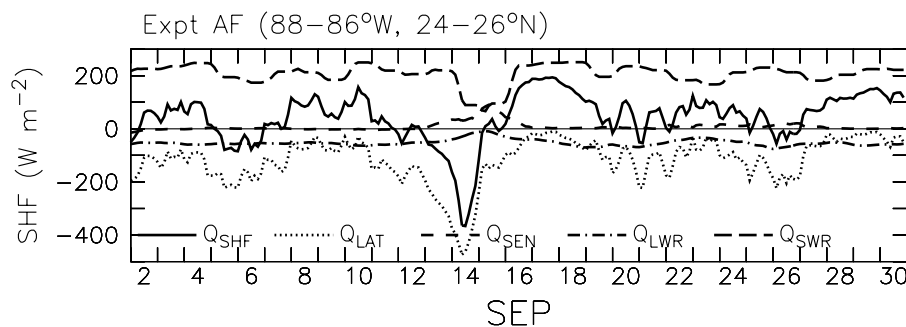
Figure 9. Box averaged three-hourly snapshots of model net surface heat flux ( Q_{SHF} ), latent heat flux ( Q_{LAT} ), sensible heat flux ( Q_{SEN} ), long-wave radiation ( Q_{LWR} ) and shortwave radiation ( Q_{SWR} ) in W m^{-2} from AF.
