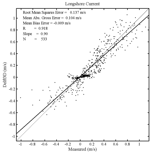
Fig. 11 – Scatter plot for longshore current excluding cases with eddy formation using Chezy with C = 55 .
