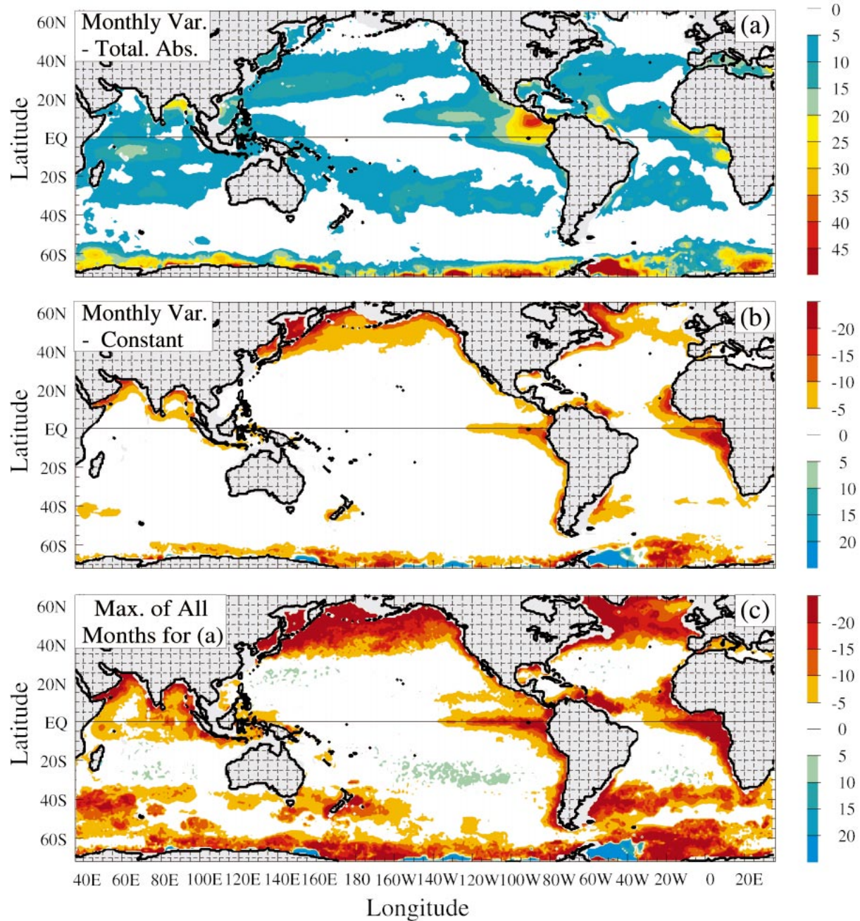
FIG. 3. Changes in PAR below the MLD as percentage of PAR at the surface: (a) annual-mean difference when using a monthly varying k_{\text{PAR}} relative to complete PAR absorption within the mixed layer (i.e., the effect of ignoring k_{\text{PAR}} ), (b) annual-mean difference when using a monthly varying k_{\text{PAR}} relative to k_{\text{PAR}} = 0.06 \text{ m}^{-1} , and (c) largest difference of all 12 months for case (b), indicating where using a monthly k_{\text{PAR}} can make a large difference in model simulations.
