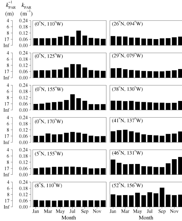
FIG. 5. Climatological monthly mean of k_{\text{PAR}} at the locations given in Tables 2 and 3. Note that x -axis labels are written for every other month.
