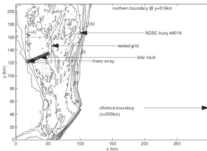
Fig. 14 — Bathymetry and data locations for Test 4
