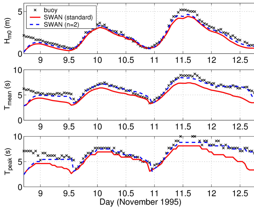
Fig. 21 — Time series comparisons for average height ( H_{m0} ), average wave period ( T_{\text{mean}} ), and peak wave period ( T_{\text{peak}} ) between SWAN and NDBC buoy 45007
