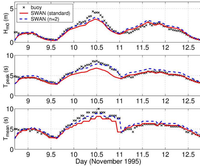
Fig. 20 — Time series comparisons for average height ( H_{m0} ), average wave period ( T_{\text{mean}} ), and peak wave period ( T_{\text{peak}} ) between SWAN and NDBC buoy 45002
