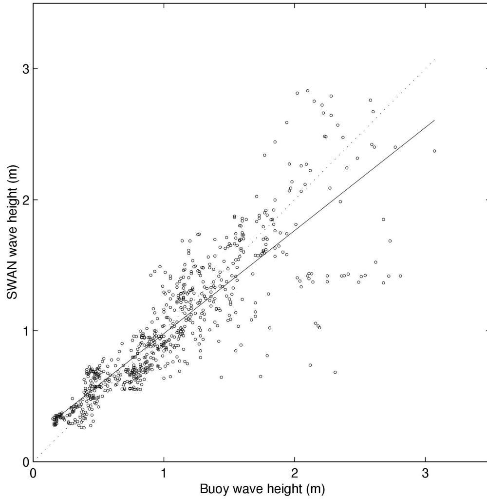
Fig. 24 — Scatterplot demonstrating the positive correlation for wave height (m) between SWAN and NDBC buoy 42040
