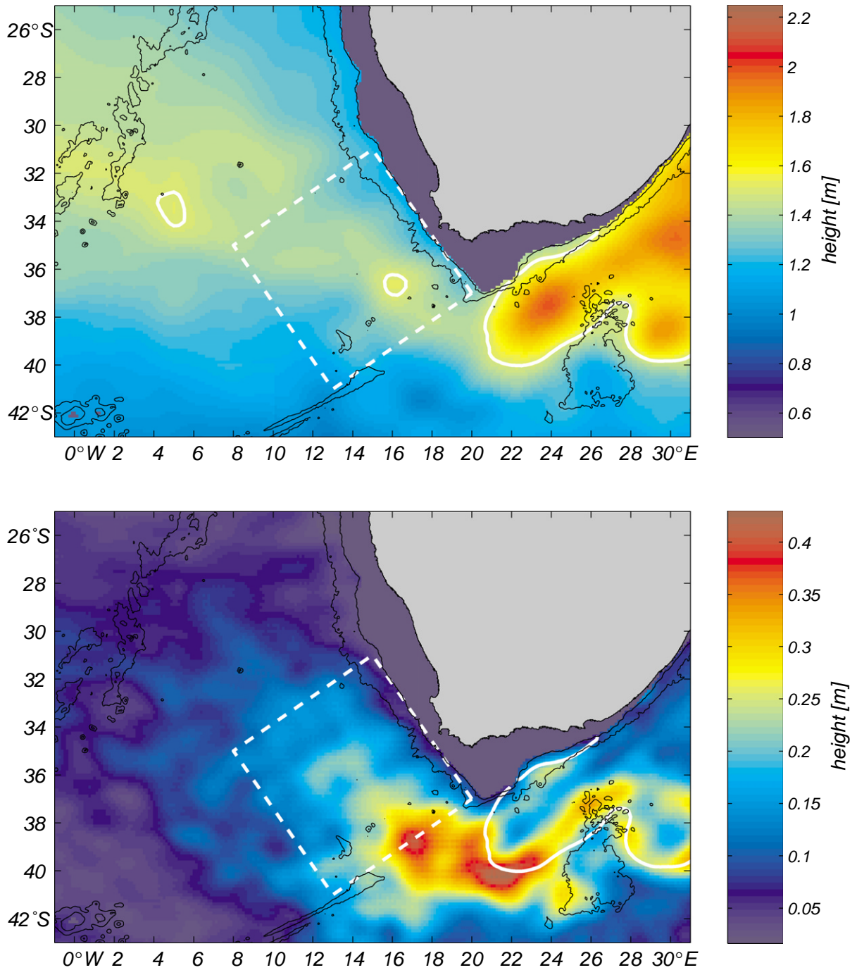
Fig. 4. Three-year mean (top) and standard deviation (bottom) from MODAS-2D SSH data. White contours in both plots give the position of the 1.5 m mean SSH. The dashed white box outlines the Cape Caudron.
