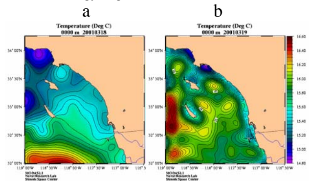
Fig. 1. MODAS nowcast field from two consecutive days: a) persistent cloud coverage, b) clear day. Due to the closeness of the coast, no altimetry data are assimilated.
