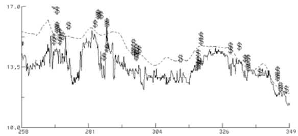
Fig. 6. Comparison between the Buoy #46042 and the MCSST data. Same as Fig. 5. (September 15 – Dec 15, 2001).
