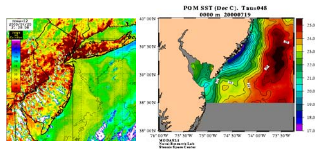
Fig. 3: Comparison between the SST from remote sensing and the 48-hour forecast from MODAS-NRLPOM.
