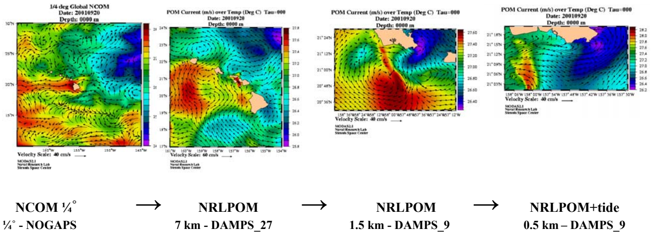
Fig. 2. A coupling/nesting procedure. See text for definition of terms.
