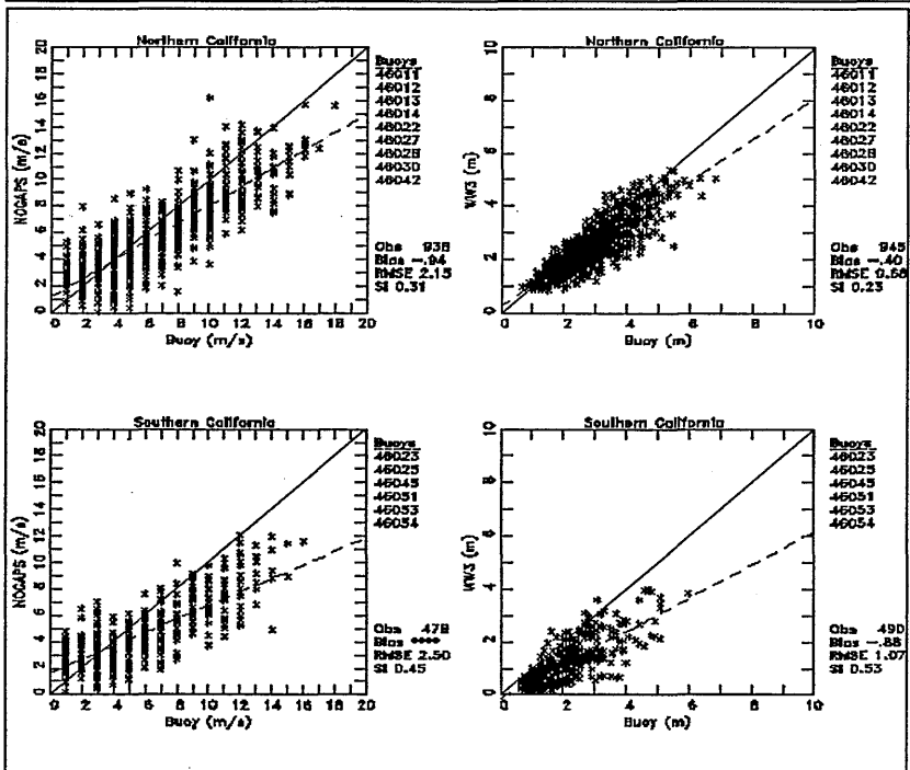
Fig. 5. FNMOG comparison for January 2002. These are the operational global wind and wave products (analyses) compared to buoys, by region. This is one of several comparisons that are made monthly. a) the “northeast Pacific” and “Gulf of Alaska” grouping, b) the “northern California” and “southern California” buoy groupings.
